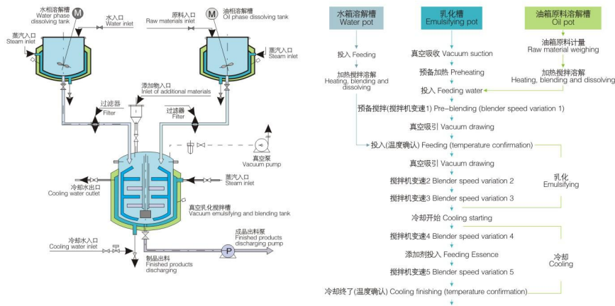
真空乳化机工艺流程 FLOW CHART OF VACUUM EMULSIFYING MIXER
